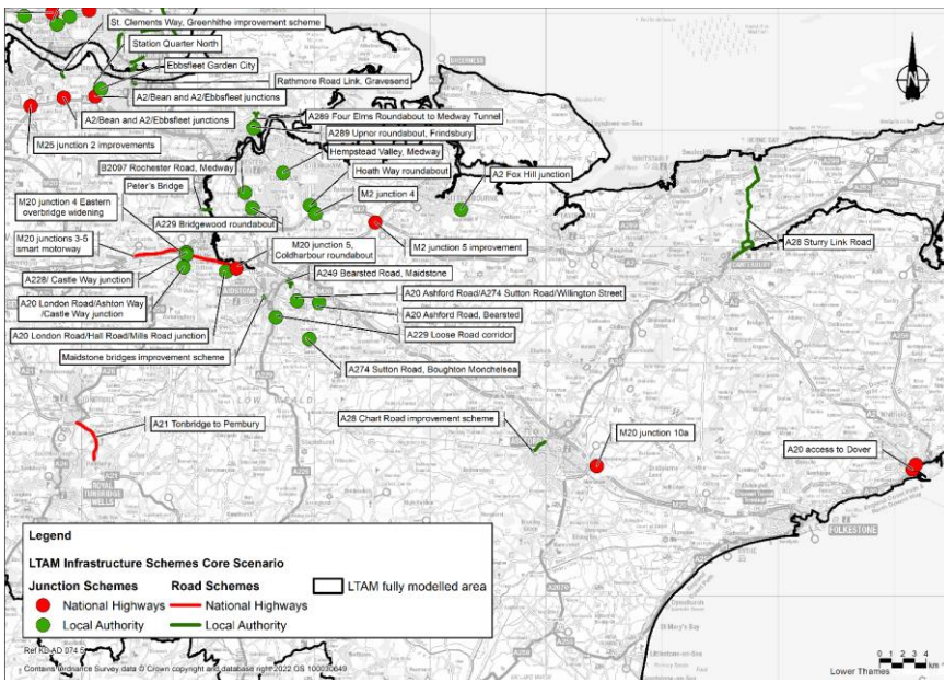
Plate 5.4 Future highway schemes (1 of 3)
