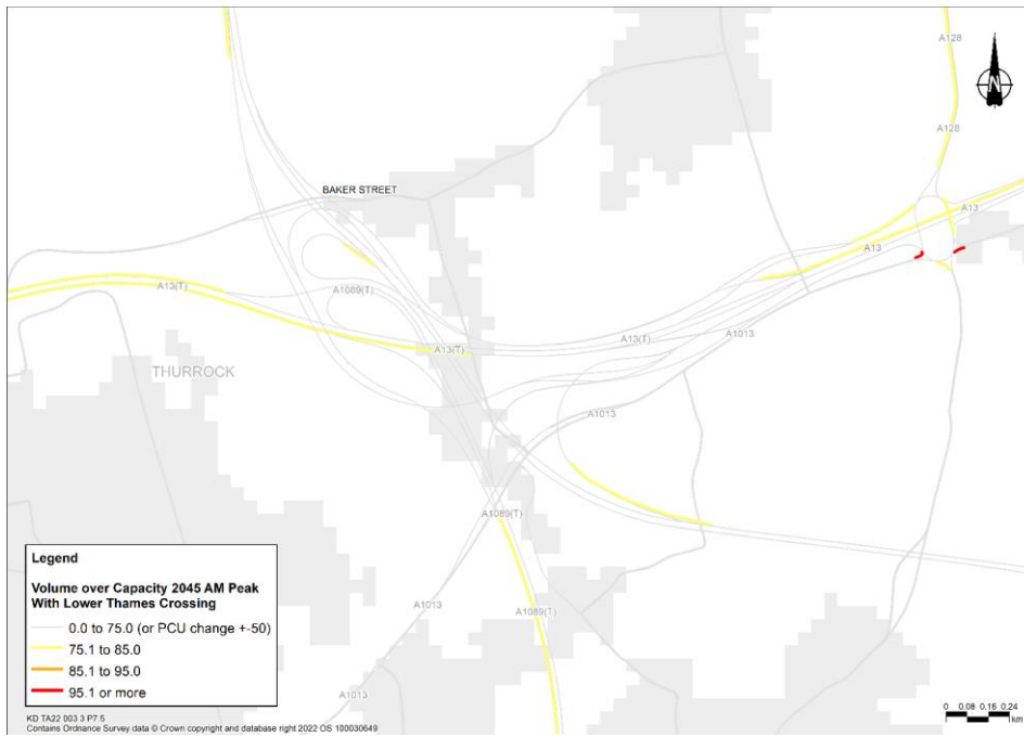
Plate 7.5 Volume to capacity at the A13/A1089/A122 Lower Thames Crossing junction – AM peak 2045
