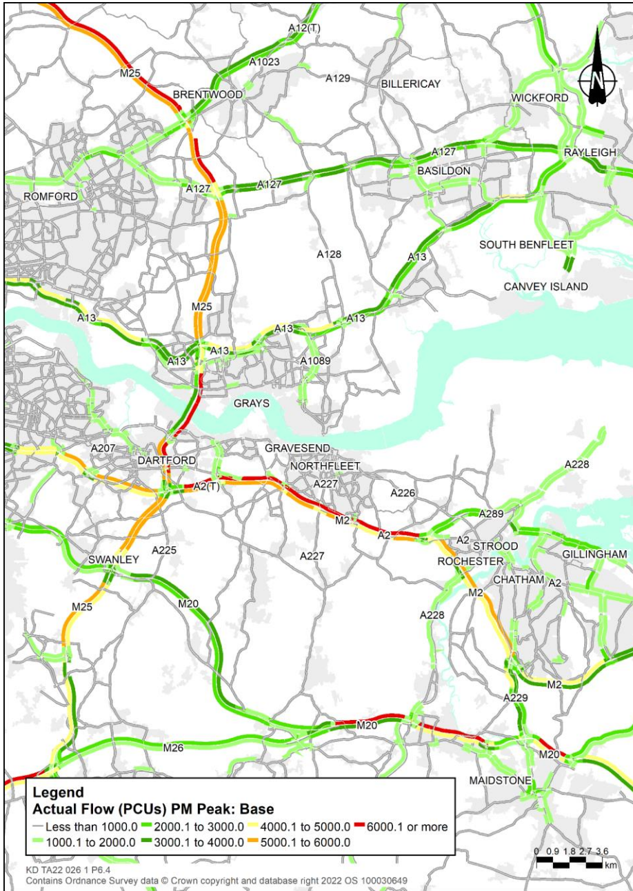
Plate 6.4 Baseline flows 2016 PM peak
